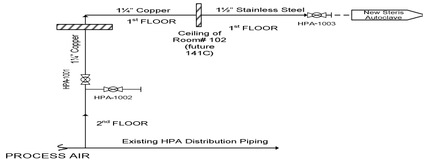
Process Air Tie-In for new Steris Autoclave Project
