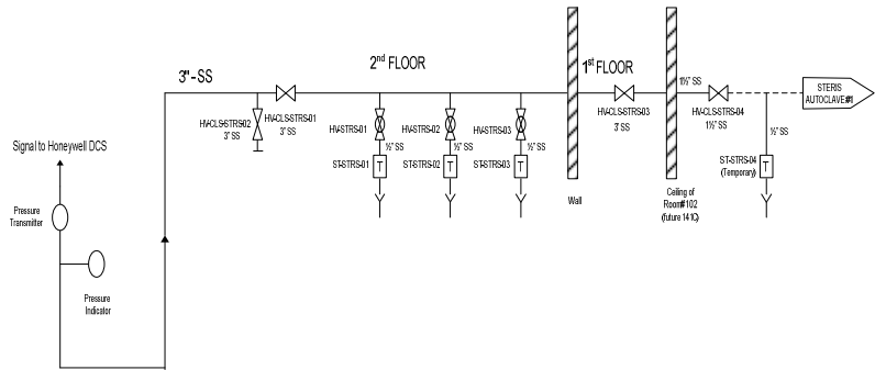
Clean Steam System Tie-In for New Steris
